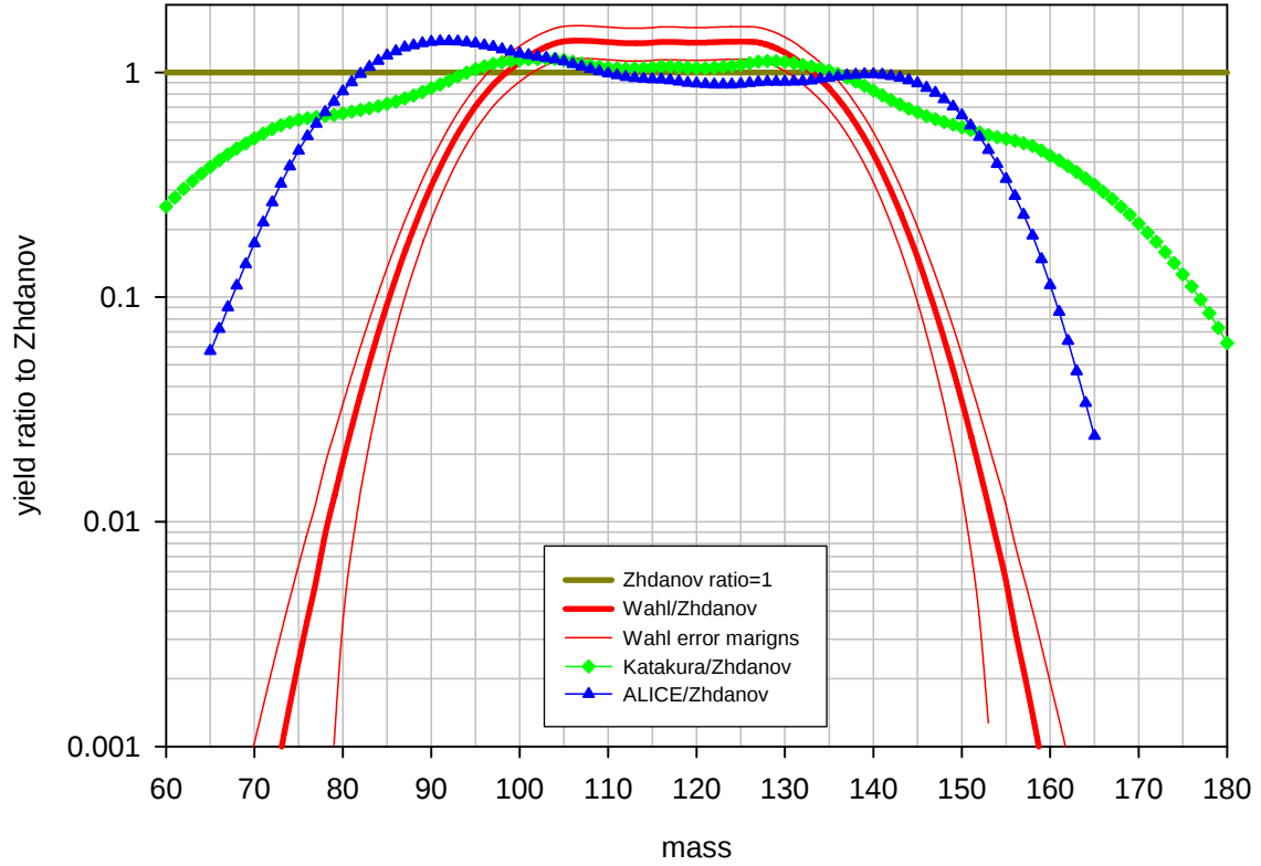
Benchmark B: ^{244}\text{Cm} at 160 MeV, post neutron emission yield ratios to Zhdanov's data
